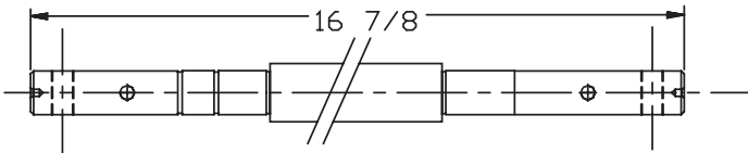
SHAFT "B"
