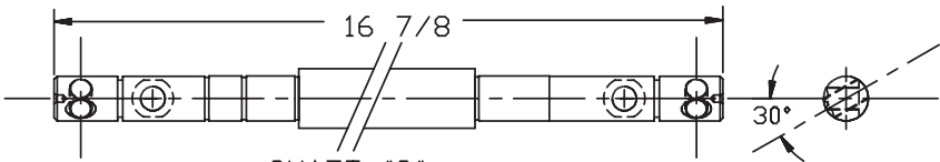
SHAFT "C"
